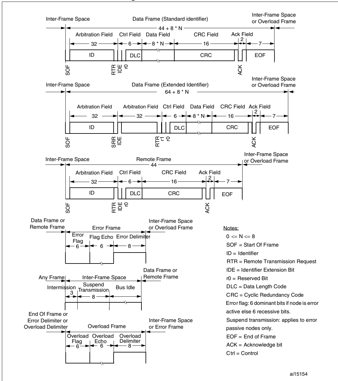
Figure 347. CAN frames
