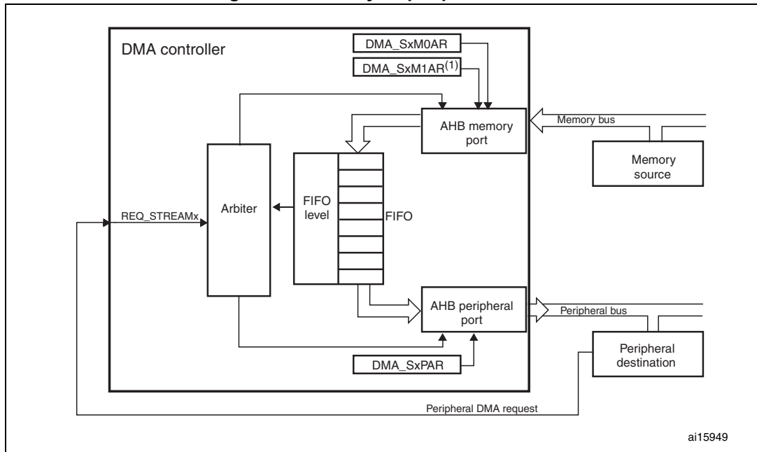
Figure 37. Memory-to-peripheral mode
