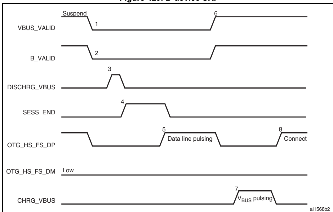
Figure 429. B-device SRP
