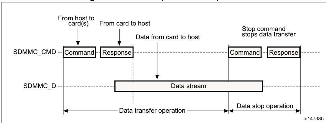
Figure 324. SDIO sequential read operation
