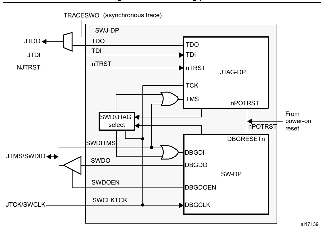
Figure 484. SWJ debug port
