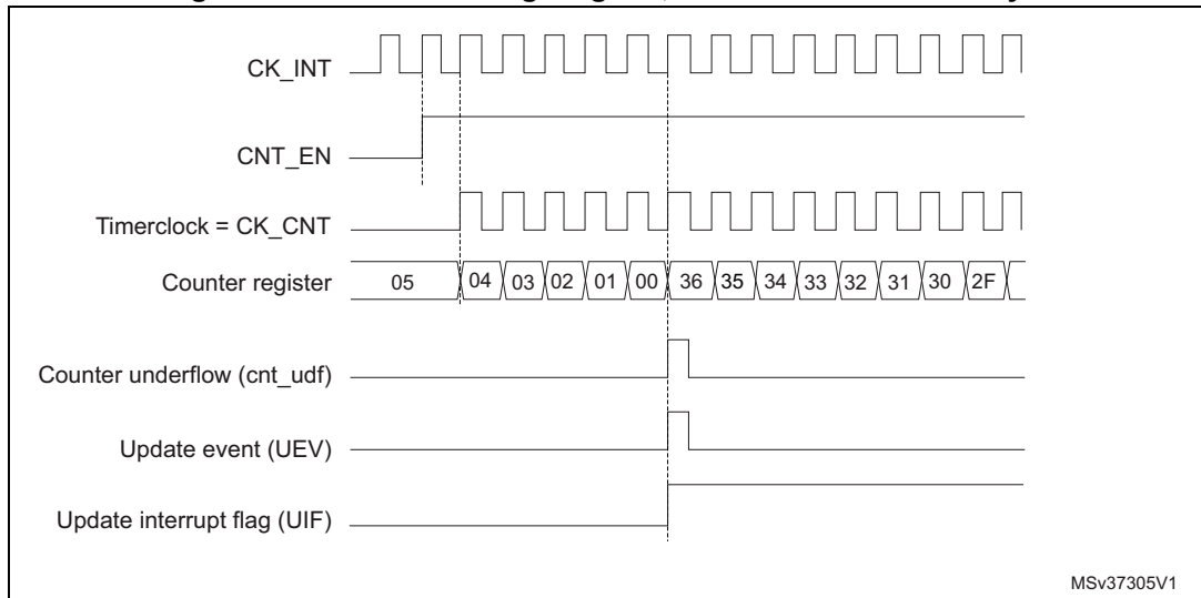
Figure 144. Counter timing diagram, internal clock divided by 2
