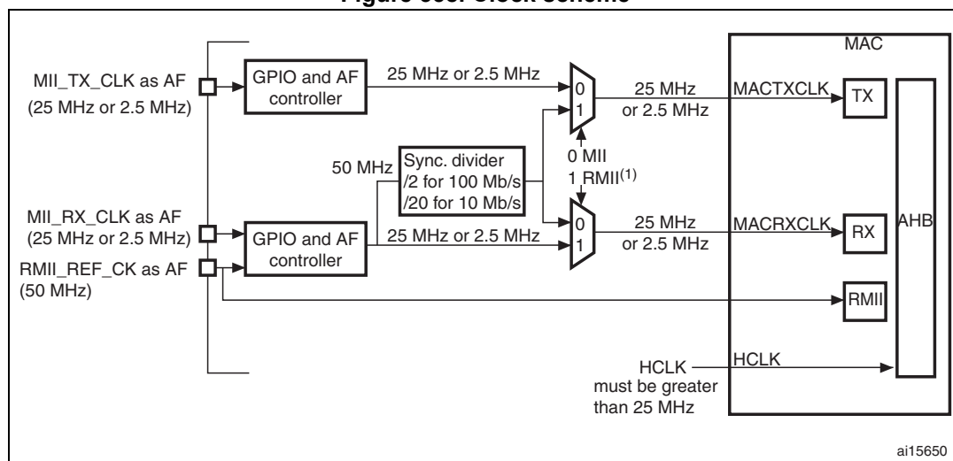
Figure 358. Clock scheme
