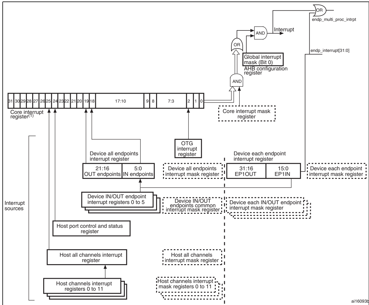
Figure 412. Interrupt hierarchy
