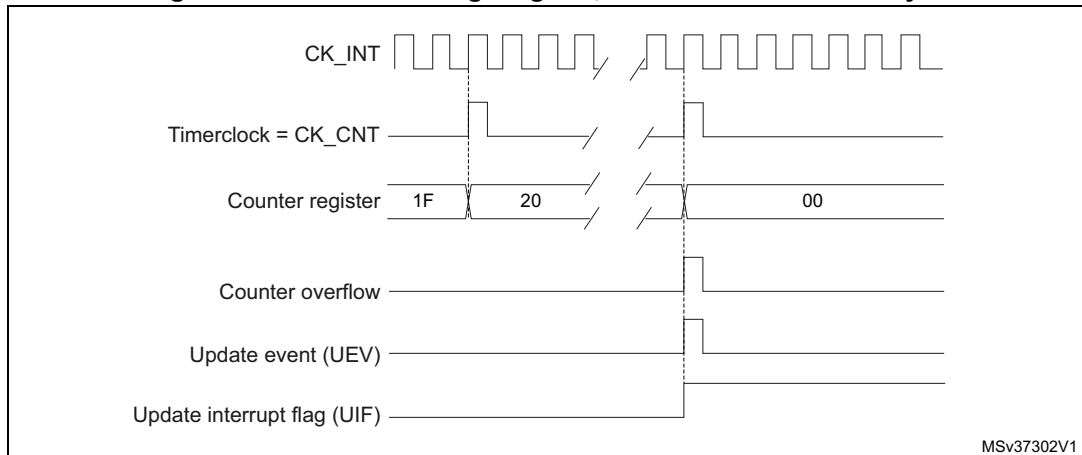
Figure 141. Counter timing diagram, Update event when ARPE=0 (TIMx_ARR not preloaded)
